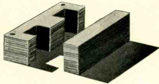
"E" and "I" punchings of Hipernik and Conpernik. These are normally mated with related shapes to form magnetic circuits through coils.
