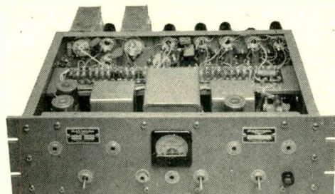
SCR-3B Single-Channel Receiver
