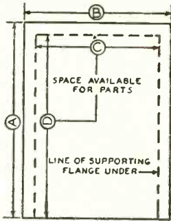
DECK PLATE PLAN-FIG. 1
