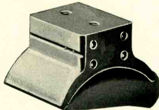
Motor pole for fractional horsepower motor made from Hipernik alloy laminations. Low coercive force assures precise positioning of d-c meters used in mechanical control applications.
