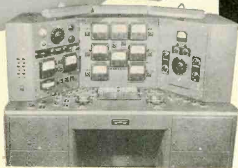
R.F. Universal Power Output Test Set built for Evans Signal Laboratories. Measurements from 20 to 4000 watts; from 2.5 mc to 60 mc.
