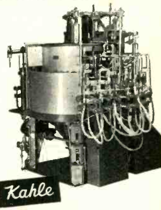
#1414 CATHODE RAY TUBE BUTTON STEM MACHINE
