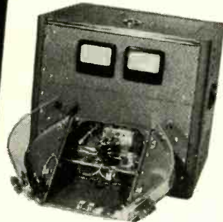
210 Type Flyback Coil Test Set
